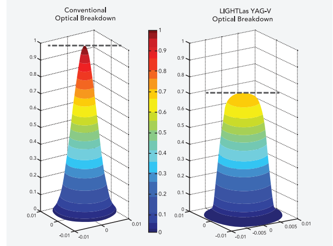
LIGHTLas YAG-V Crystal Q-Switch Gaussian Profile
